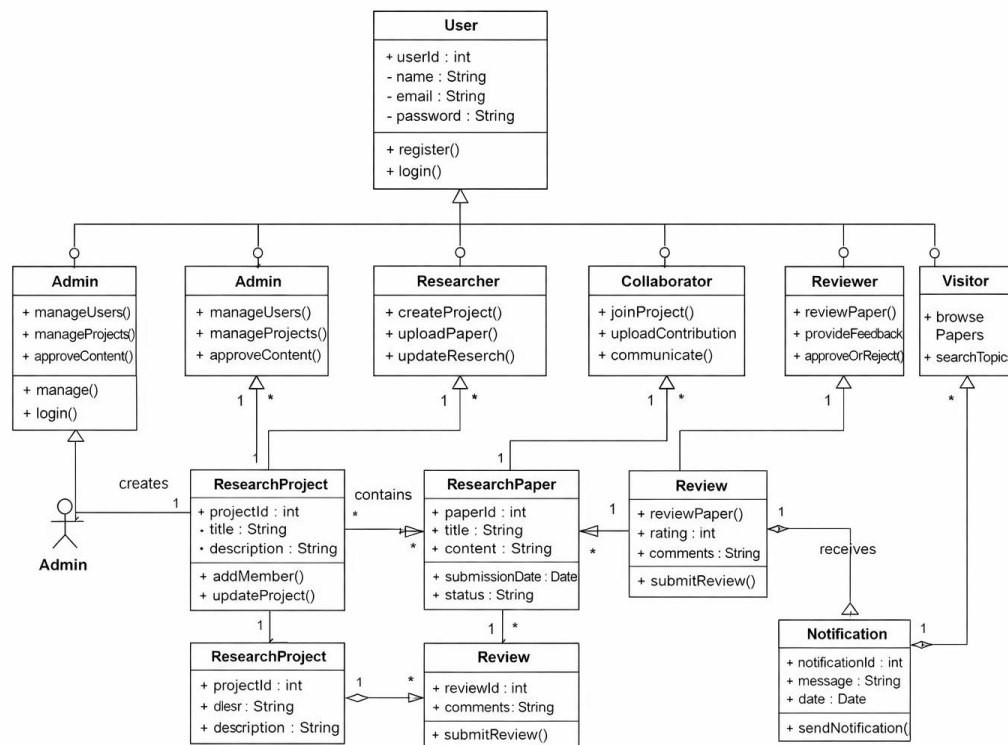
Research and Collaboration System - Class Diagram
